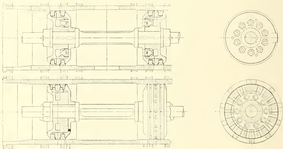
FIG. 49—G. HUGHES'S PISTON VALVE, L. & Y. RLY.
