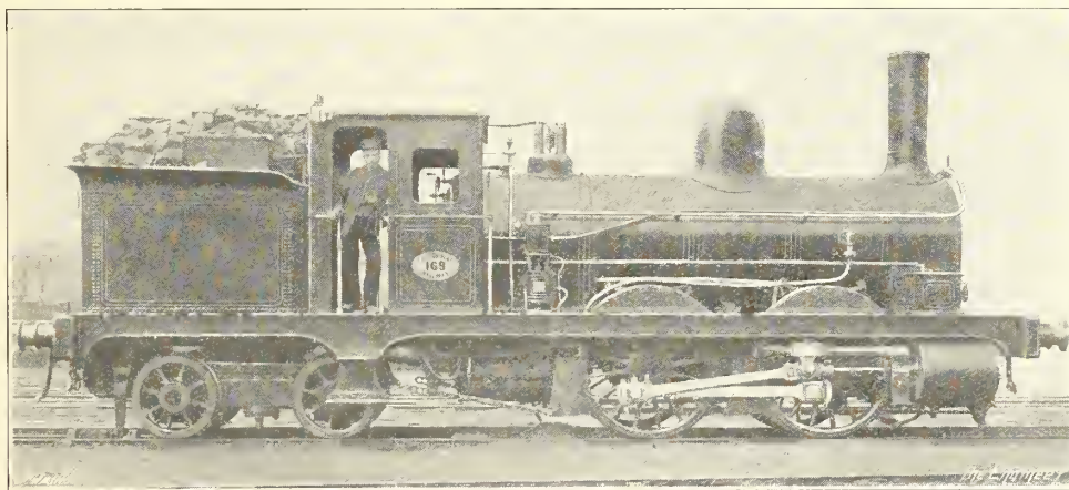
FIG. 262—CALEDONIAN RAILWAY TANK ENGINE. 1873-74
