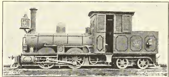
FIG. 303—METRE GAUGE ENGINE FOR INDIA, 1872
