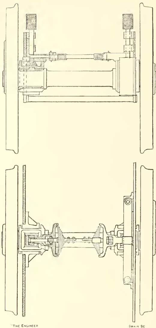
FIG. 209—CAILLET'S MOVABLE AXLE
