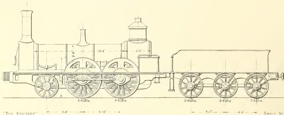
FIG. 56—BRISTOL AND BIRMINGHAM RAILWAY ENGINE, VULCAN FOUNDRY, 1846
