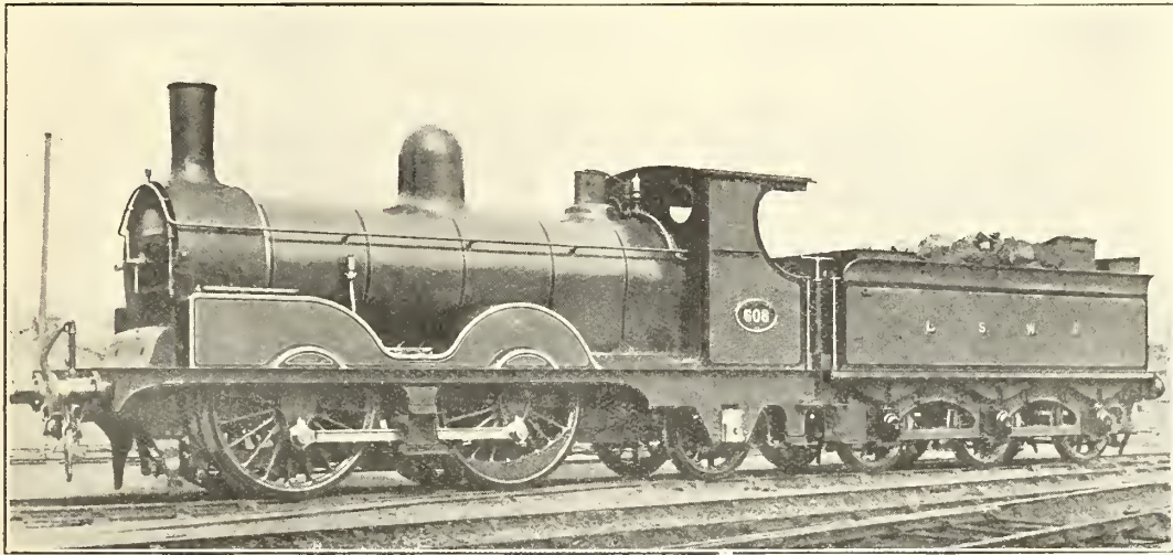
FIG. 344—W. ADAMS'S FRONT COUPLED ENGINE, LONDON & SOUTH-WESTERN RLY., 1887 [Photo. Locomotive
