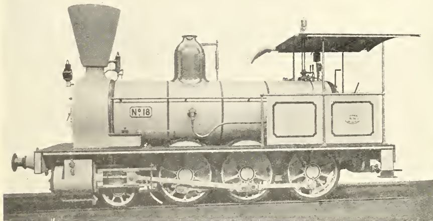
FIG. 239—KITSON'S ENGINE FOR QUEENSLAND, 1866
