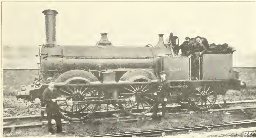
FIG. 191—J. E. McCONNELL'S TANK ENGINE FOR THE L. & N.W. RLY., 1862 (Photo. Locomotive)
