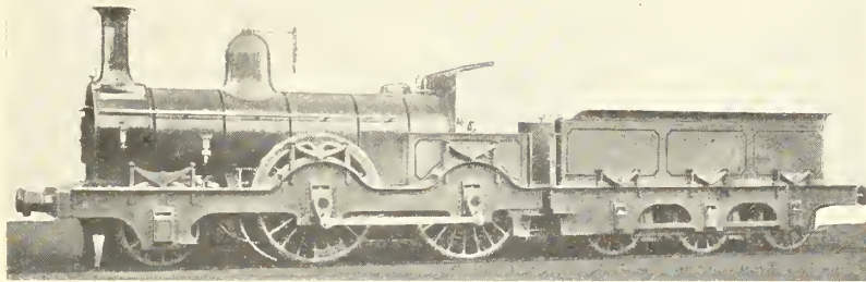
FIG. 244—M. KIRTLEY'S EXPRESS ENGINE, MIDLAND RLY., BUILT BY NEILSON & CO., 1870
