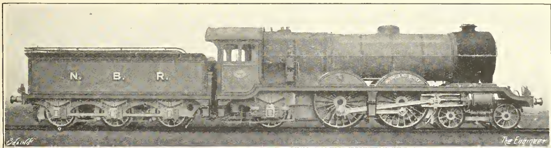
FIG. 416—W. P. REID'S "ATLANTIC" TYPE LOCOMOTIVE, NORTH BRITISH RLY. 1906-11
