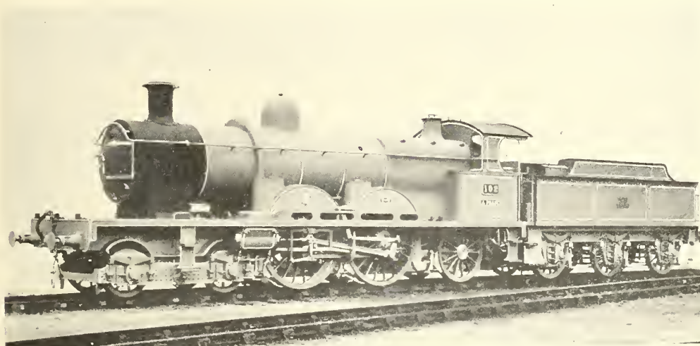
FIG. 407—DE GLEHN FOUR-CYLINDER COMPOUND LOCOMOTIVE, GREAT WESTERN RLY., 1903
