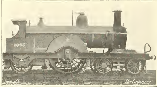
FIG. 330—S. W. JOHNSON'S SINGLE EXPRESS ENGINE, MIDLAND RLY., 1889-93
