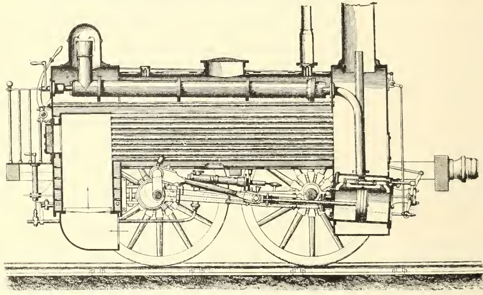
FIG. 13—STEPHENSON'S "PLANET," LIVERPOOL AND MANCHESTER RAILWAY, 1830
