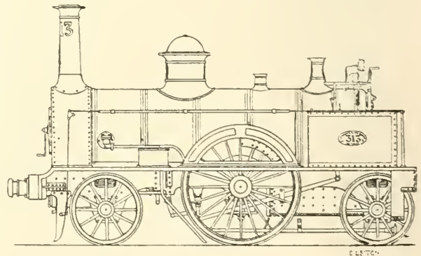
FIG. 105—L. & N.W. RLY., McCONNELL "SMALL BLOOMER," 1854-61
