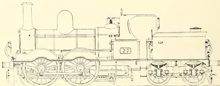
FIG. 234—A. McDONNELL'S TANK LOCOMOTIVE, G.S. & W.R., LATER DESIGN, 1871-84
