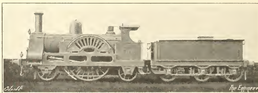
FIG. 75A—THE "CORNWALL," L. & N.W. RAILWAY, AS REBUILT 1858
