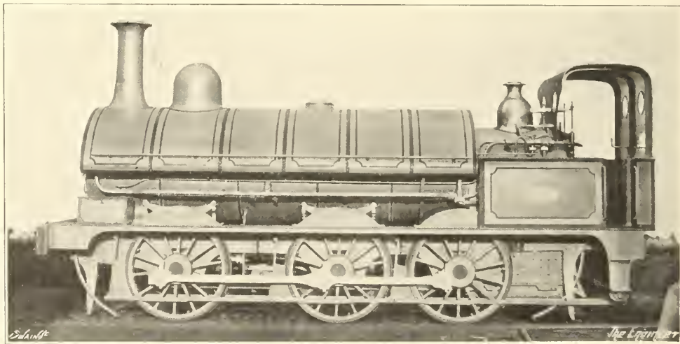
FIG. 225—SHARP, STEWART & CO.'S TANK ENGINE FOR THE BRECON & MERTHYR RLY., 1865-68
