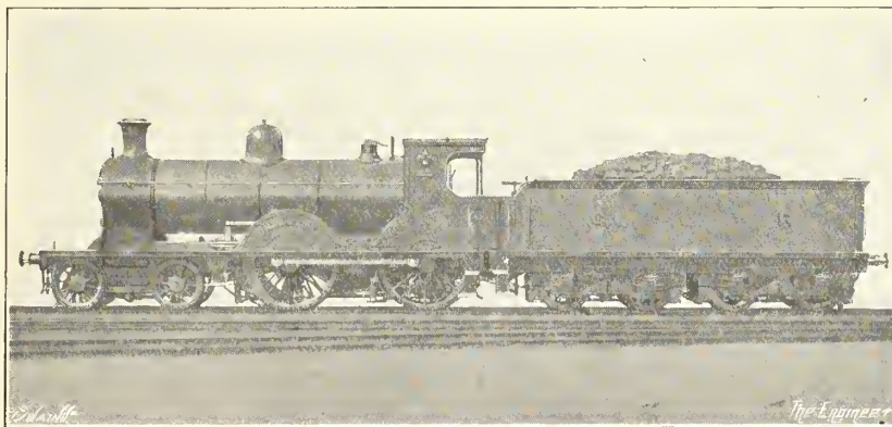
FIG. 378—J. F. McINTOSH'S "766" CLASS EXPRESS ENGINE, CALEDONIAN RLY., 1897
