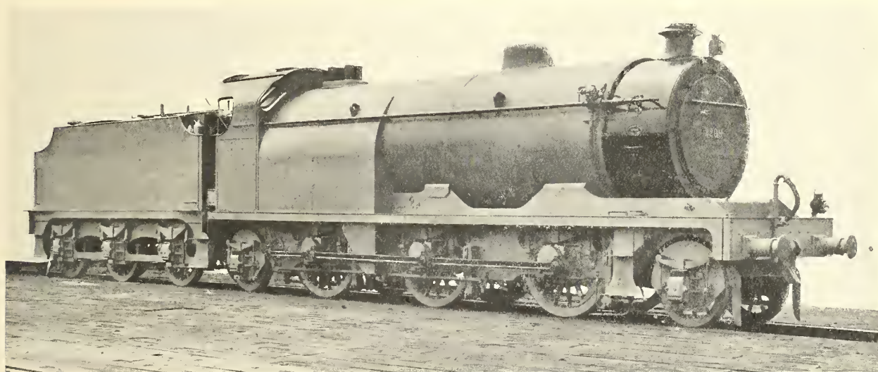
FIG. 438—SIR CECIL PAGET'S EIGHT-CYLINDER ENGINE, MIDLAND RAILWAY, 1908
