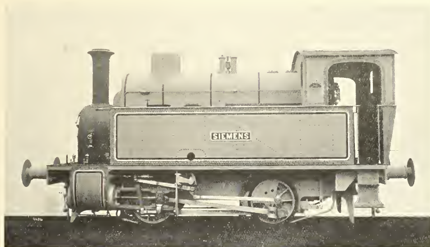
FIG. 448—BEYER, PEACOCK'S TANK ENGINE WITH BROTTAN WATER-TUBE FIRE-BOX, 1907
