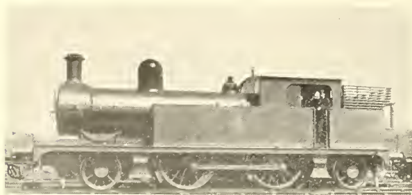
FIG. 349—ASPINALL'S 2-4-2 TANK LOCOMOTIVE, L. & Y. RLY., 1889-1901
