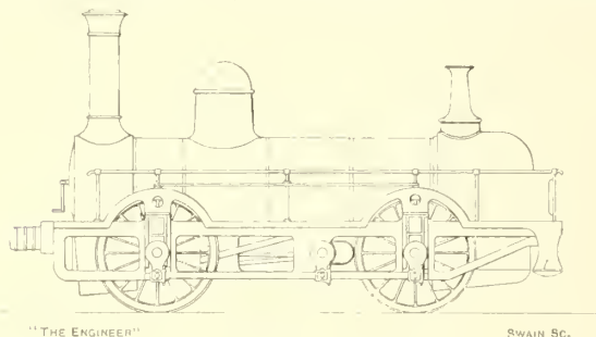
FIG. 89—VULCAN FOUNDRY LOCOMOTIVE, SHREWSBURY & CHESTER RLY., 1848
