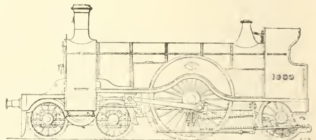
FIG. 368—P. STIRLING'S SGL. SINGLE EXPRESS ENGINE. GREAT NORTHERN RLY., 1894.
