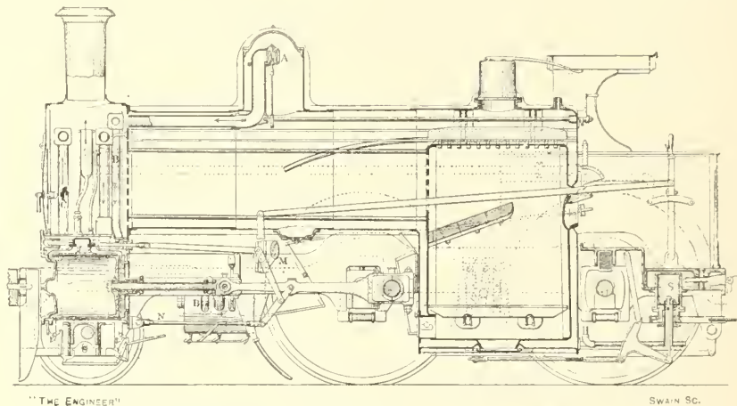
FIG. 308.—SECTIONAL ELEVATION OF L. & N.W. COMPOUND, 1882-83
