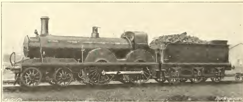
FIG. 341—H. SMELLIE'S PASSENGER LOCOMOTIVE, G. & S.W.R., 1888-89
