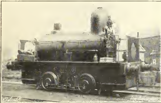
FIG. 293—F. W. WEBB'S L. & N.W.R. SHUNTING ENGINE, 1880-82
