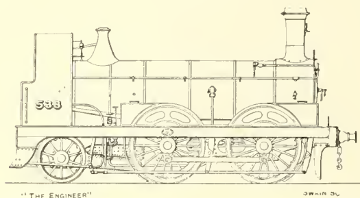
FIG. 220—P. STIRLING'S GREAT NORTHERN ENGINE, 1867-79
