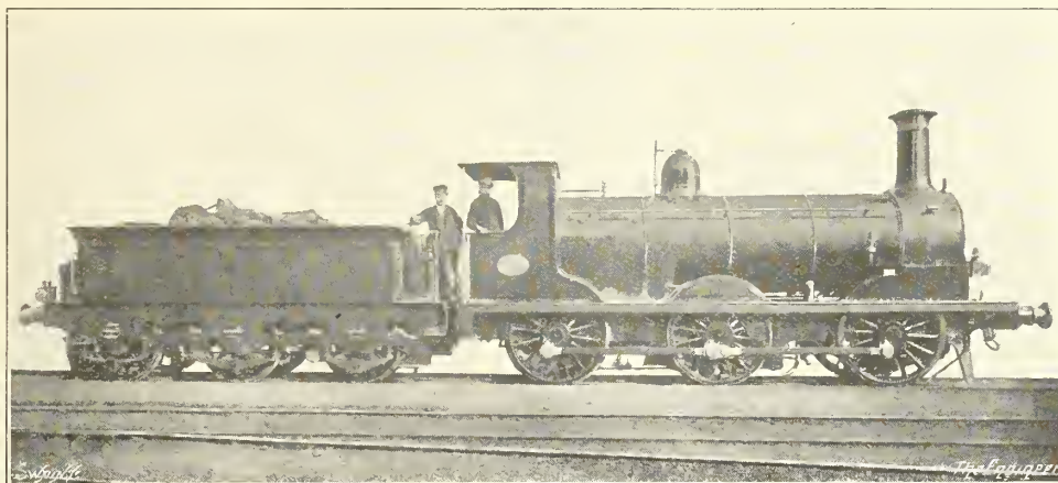
FIG. 265—W. STROUDLEY'S L.B. & S.C.R. GOODS ENGINE, 1873
