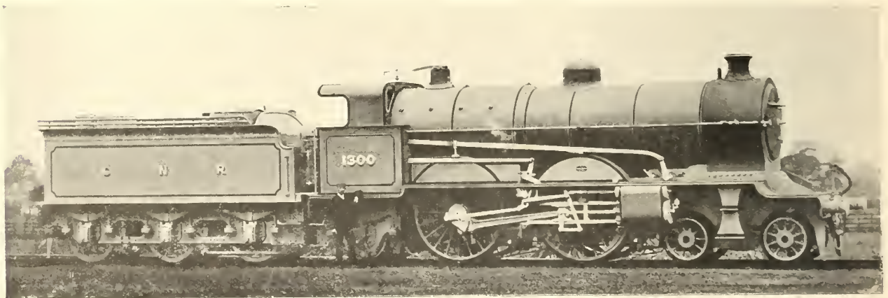
FIG. 409—VULCAN FOUNDRY FOUR-CYLINDER COMPOUND EXPRESS ENGINE, GREAT NORTHERN RLY., 1905
