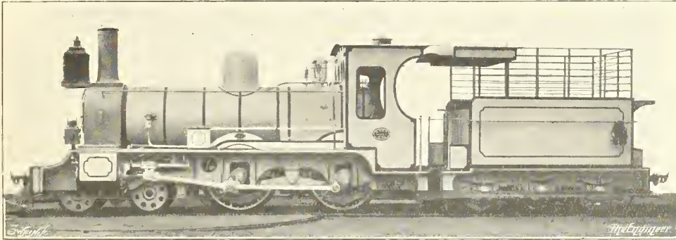
FIG. 306—INDIAN STATE RLYS., CLASS "O," AND BENGAL AND NORTH-WESTERN RLY. LOCOMOTIVE, BY VULCAN FOUNDRY, 1883
