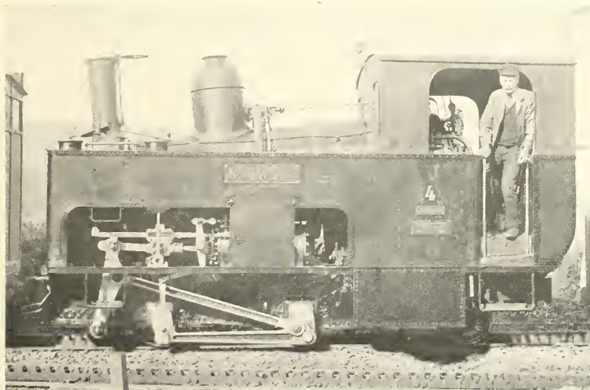
FIG. 403—RACK LOCOMOTIVE, SNOWDON MOUNTAIN RLY., 1896
