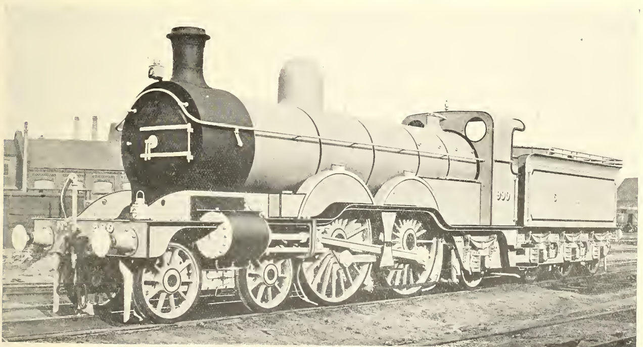
FIG. 383—H. A. IVATT'S "ATLANTIC" TYPE EXPRESS ENGINE, GREAT NORTHERN RLY., 1898
