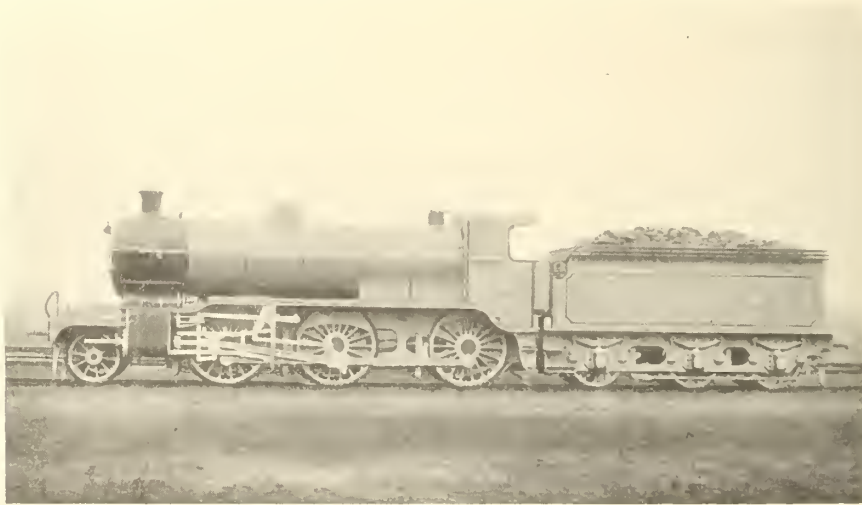
FIG. 437—H. N. GRESLEY'S MIXED TRAFFIC ENGINE, GREAT NORTHERN RLY., 1912
