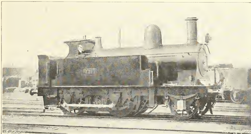
FIG. 345—W. DEAN'S TANK ENGINE, G.W. RLY., 1885 [Photo. Locomotive
