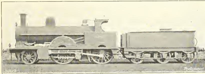
FIG. 309—"DREADNOUGHT" CLASS COMPOUND, L. & N.W.R., 1884-88
