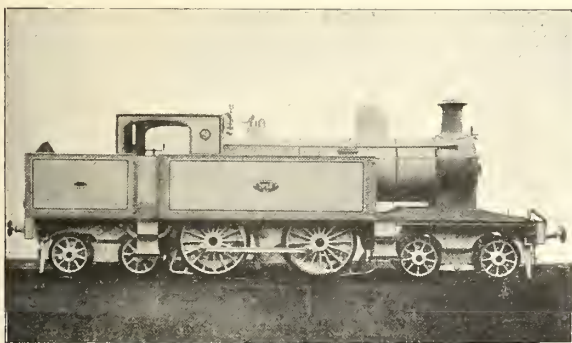
FIG. 387—BEYER, PEACOCK & CO.'S 4-4-4 TANK ENGINE, WIRRAL RLY., 1896
