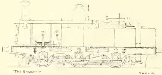
FIG. 224—R. H. BURNETT'S METROPOLITAN RAILWAY TANK ENGINE, 1868
