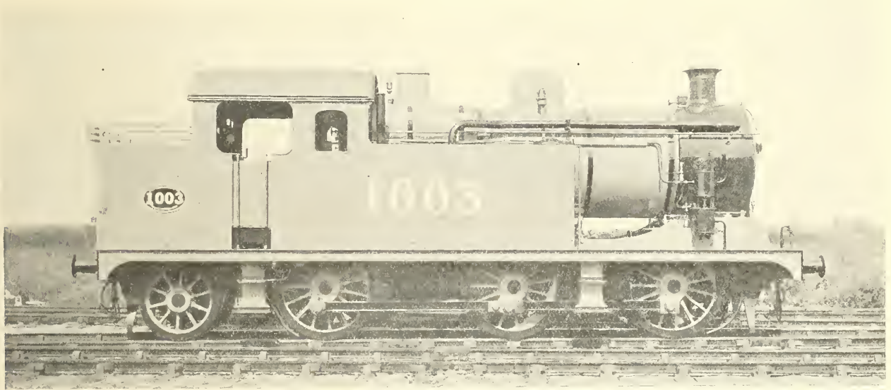
[Photo. Locomotive
