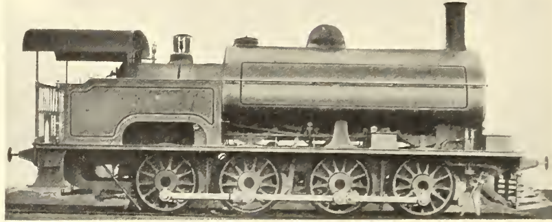
FIG. 237—EIGHT-COUPLED SADDLE TANK LOCOMOTIVE FOR THE G.I.P.R.L.Y., BY NEILSON & CO., 1879
