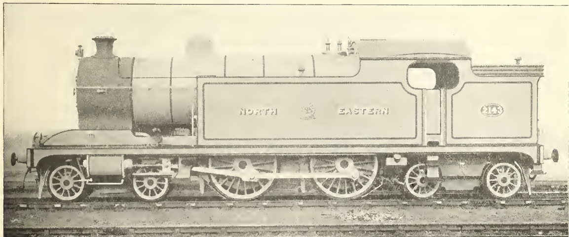
FIG. 429—SIR V. RAVEN'S THREE-CYLINDER PASSENGER TANK ENGINE, NORTH-EASTERN RLY., 1913
