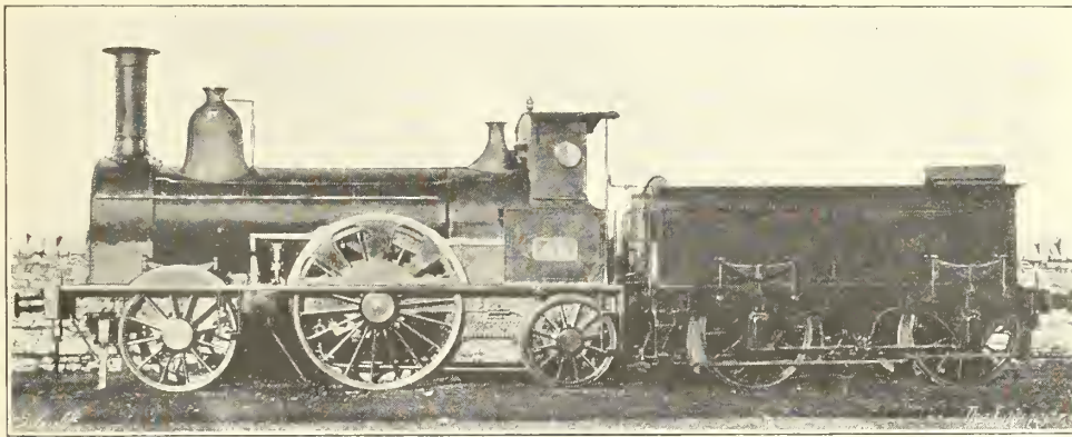
FIG. 228—J. WAKEFIELD'S G.S. & W. RAILWAY EXPRESS ENGINE, 1858-63 [Photo. Locomotive]
