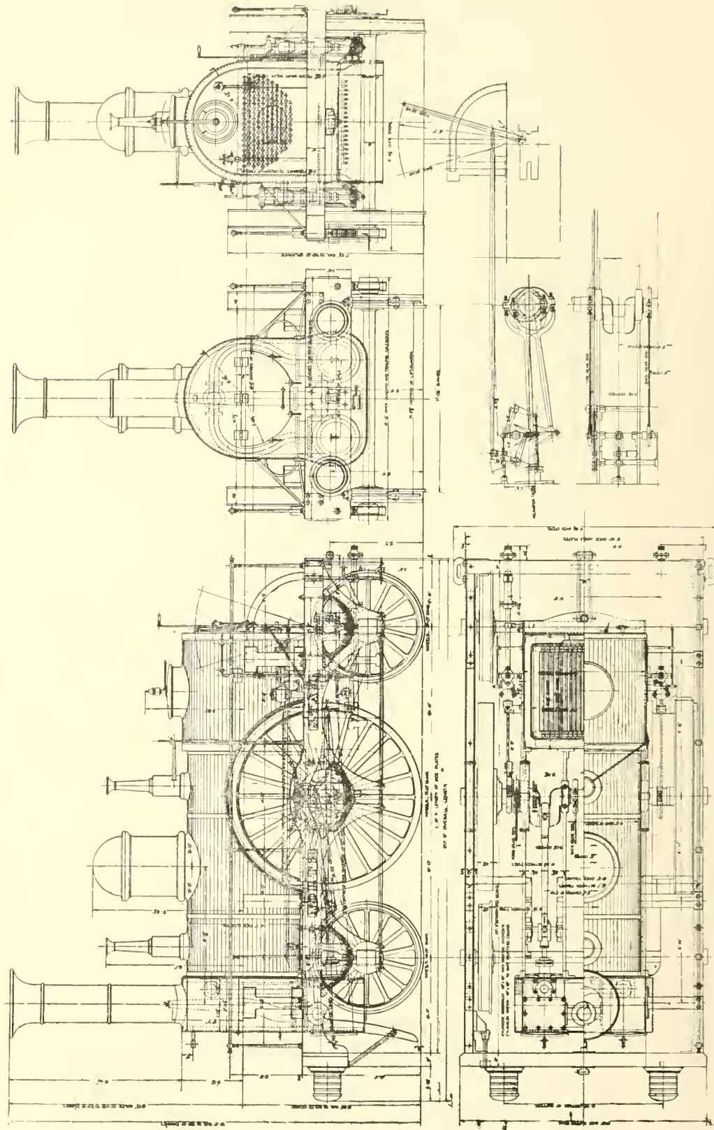
FIG. 13—GENERAL ARRANGEMENT OF THE "NORTH STAR" G.W.R. OF 1837, AS RECONSTRUCTED AT SWINDON WORKS IN 1925 Reproduced from drawing by courtesy of Mr. C. B. Collett, Chief Mechanical Engineer For a detailed description see The Locomotive , Vol. XXVII, 1926, page 10 et seq
