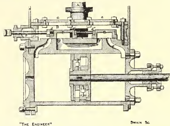
FIG. 15—CYLINDERS AND VALVES FOR STEPHENSON'S "PLANET" TYPE ENGINES, 1831
