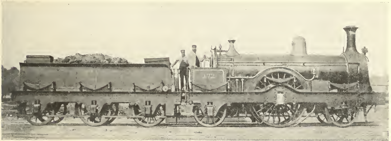
[Photo. Locomotive
