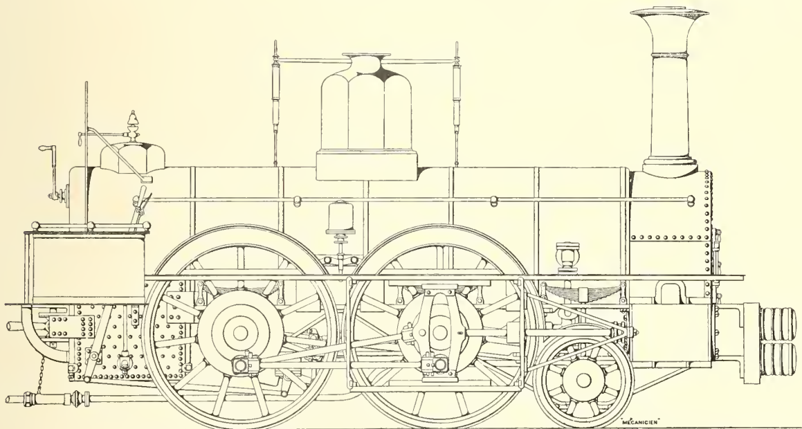
FIG. 61—2-4-0 PASSENGER ENGINE, No. 38, "ROKEBY," STOCKTON AND DARLINGTON RLY., 1847
