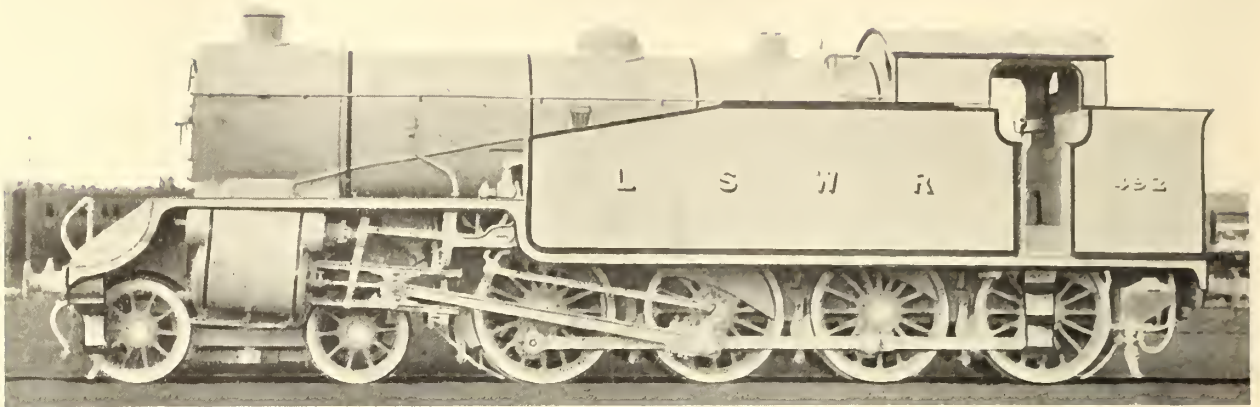
FIG. 468—R. W. URIE'S 4-8-0 SHUNTING TANK ENGINE, LONDON & SOUTH-WESTERN RLY., 1921
