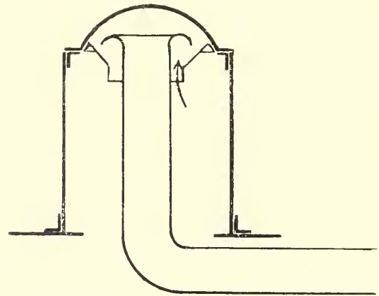
FIG. 131—R. & W. HAWTHORN'S STEAM DOME
