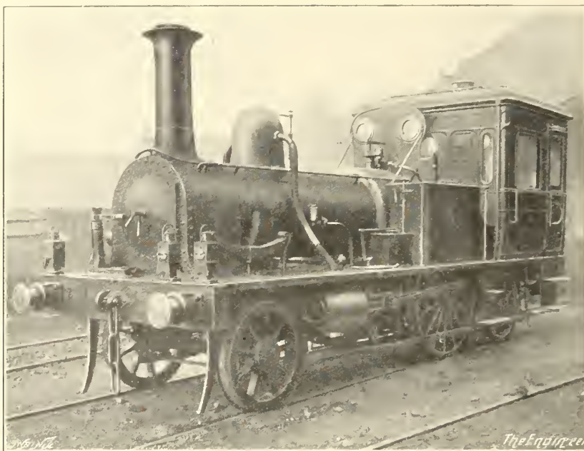
FIG. 95—TANK ENGINE, BY NEILSON & CO., EDINBURGH & GLASGOW RLY., 1859
