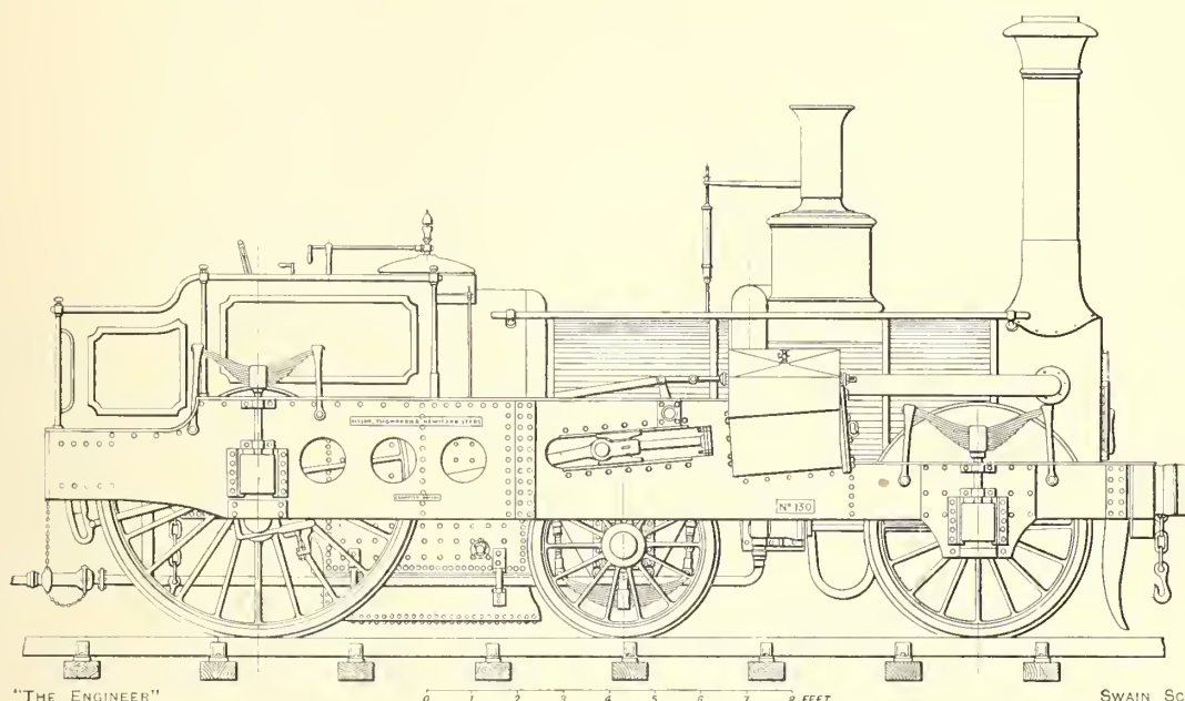
FIG. 74—CRAMPTON ENGINE BY KITSON, THOMPSON & HEWITSON, MIDLAND RAILWAY, 1848
