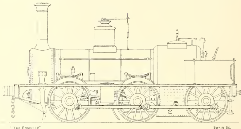
FIG. 85—KITSON, THOMPSON & HEWITSON'S ENGINE, LEEDS & THIRSK RLY., 1848
