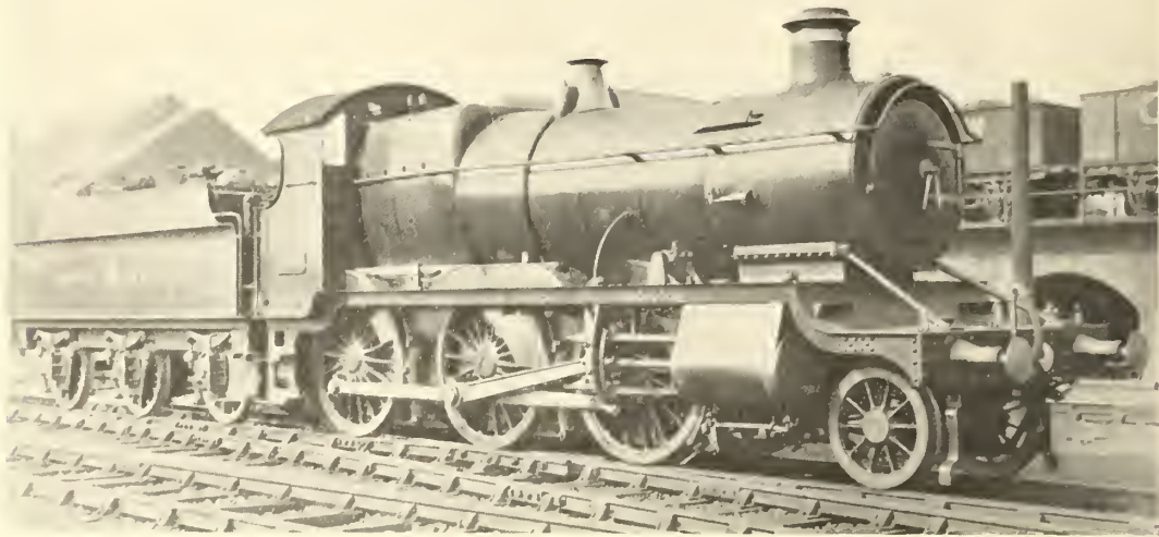
FIG. 436—G. J. CHURCHWARD'S "MOGUL" MIXED TRAFFIC ENGINE, GREAT WESTERN RLY., 1911
