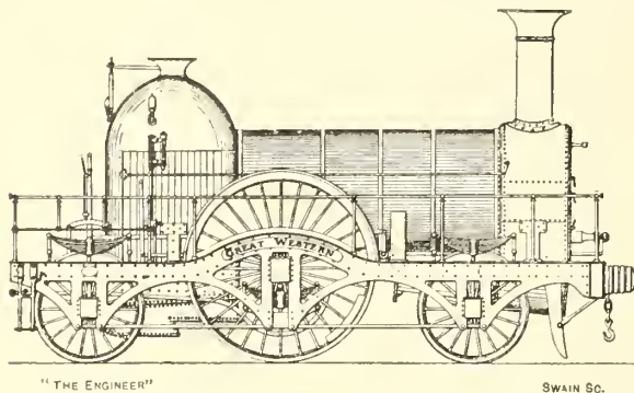
FIG. 67.—GOOCH'S BROAD GAUGE "GREAT WESTERN," BUILT AT SWINDON, 1846
