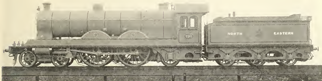
FIG. 410—W. WORSDELL'S FOUR-CYLINDER COMPOUND EXPRESS LOCOMOTIVE, NORTH-EASTERN RLY., 1906
