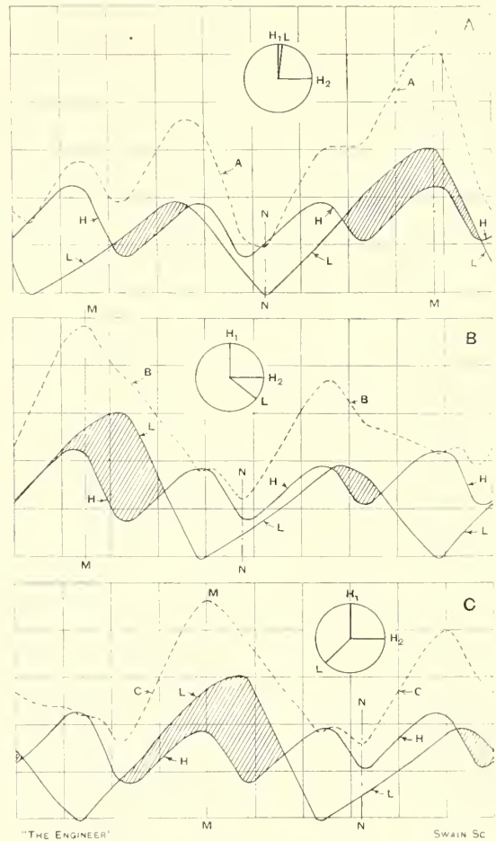
FIG. 311—CURVES OF CRANK EFFORT, L. & N.W.R. COMPOUND ENGINES
