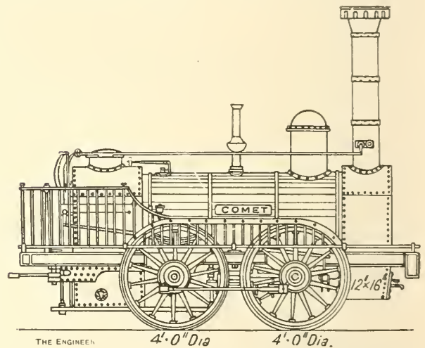
FIG. 26—HAWTHORN'S ENGINE "COMET," NEWCASTLE AND CARLISLE RAILWAY, 1835
