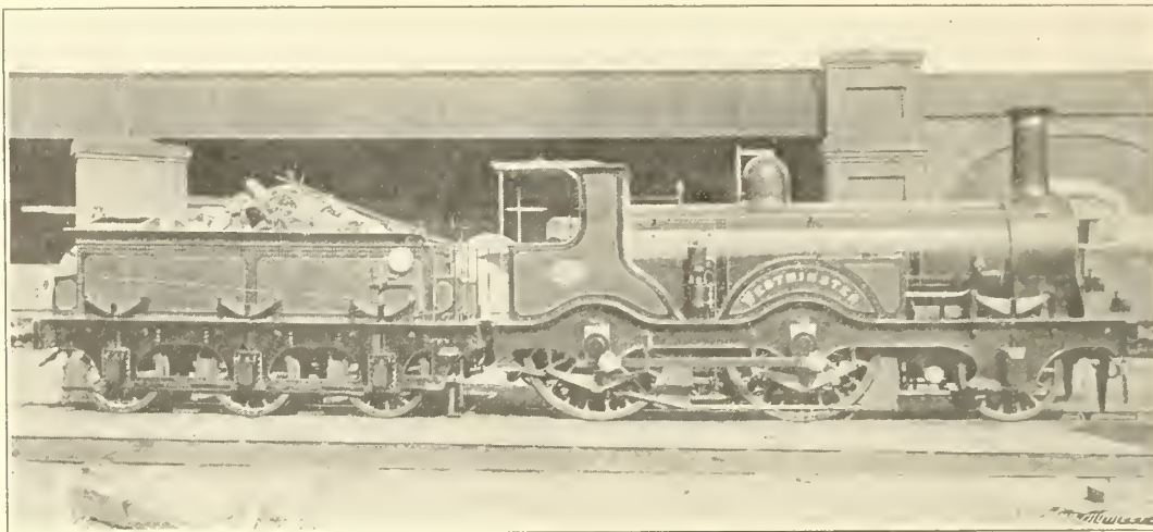
FIG. 248—STROUDLEY'S EXPRESS LOCOMOTIVE, L.B. & S.C. RLY., 1872-75 [Photo. Locomotive
