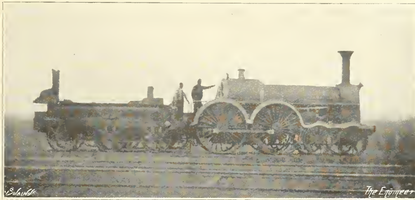
FIG. 138—G.W.R. BROAD GAUGE LOCOMOTIVE "CŒUR DE LION," BY D. GOOCH, BUILT BY R. STEPHENSON & CO., 1855 (From a photo lent by Mr. H. V. Pegg)
