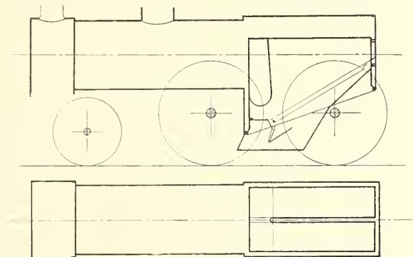
Fig. 165—Cudworth's System, South-Eastern Railway COAL BURNING FIRE-BOXES, 1852-59
