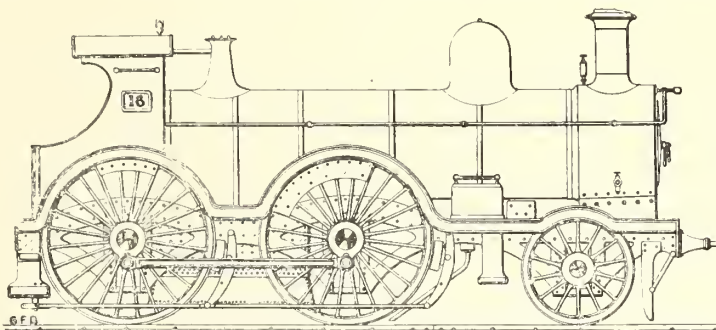
FIG. 337—BROAD-GAUGE CONVERTIBLE EXPRESS ENGINE, G.W.R., 1888
