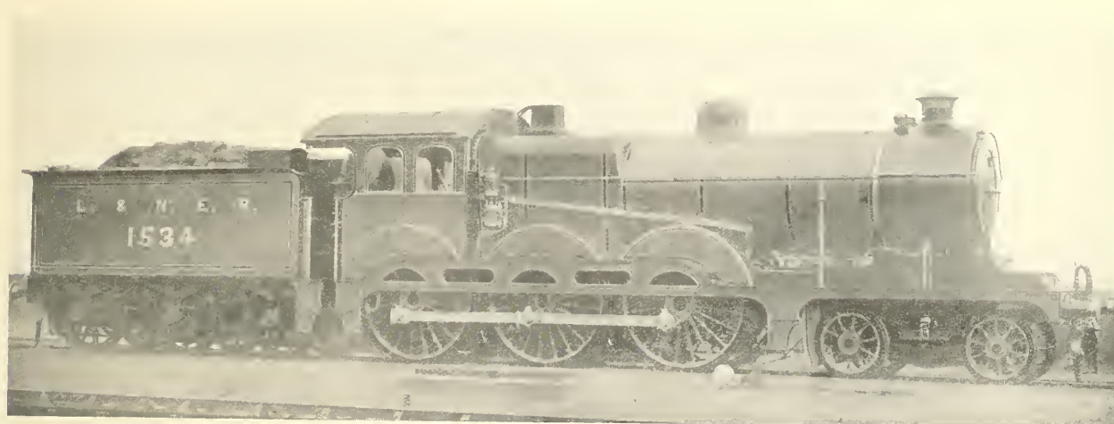
FIG. 419—S. D. HOLDEN'S 4-6-0 EXPRESS ENGINE, GREAT EASTERN RLY., 1911
