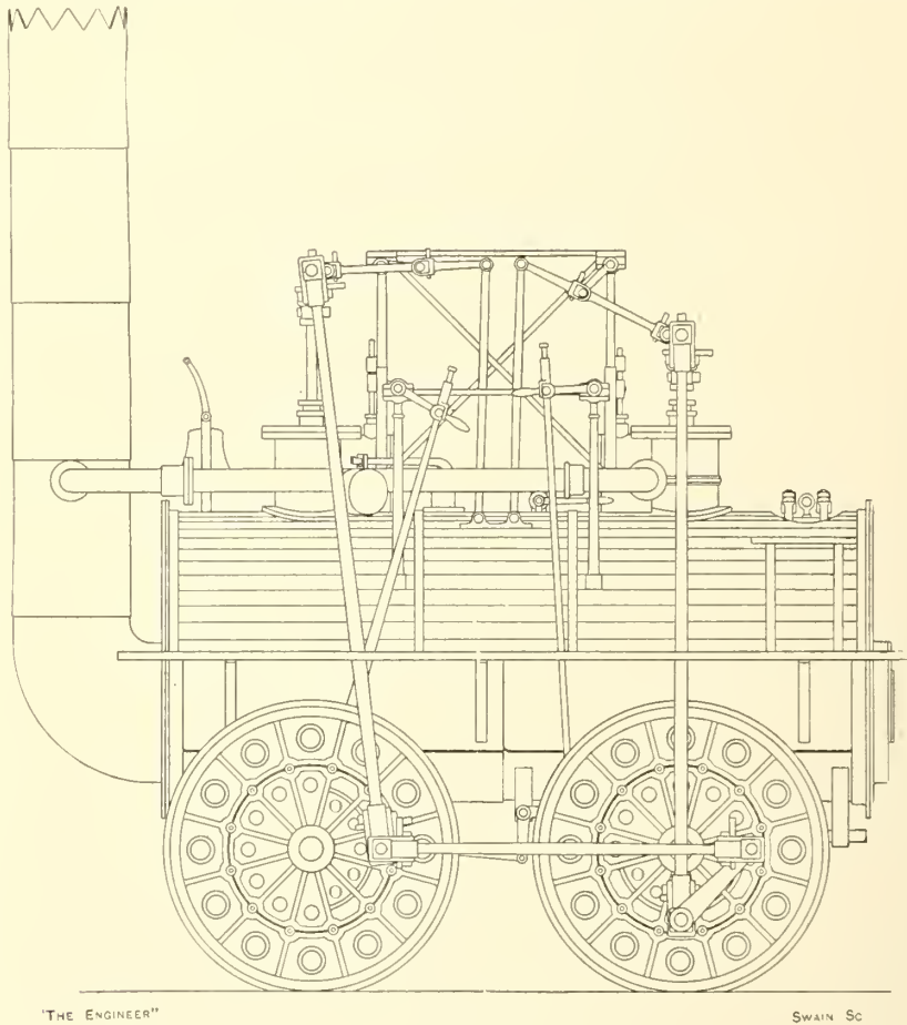
FIG. 2—"LOCOMOTION NO. 1"—STOCKTON AND DARLINGTON RAILWAY, 1825.
