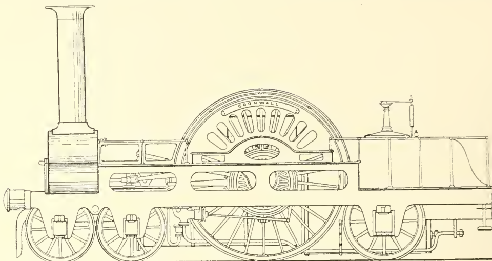
FIG. 75—F. TREVITHICK'S "CORNWALL," L. & N.W. RAILWAY, AS BUILT 1847
