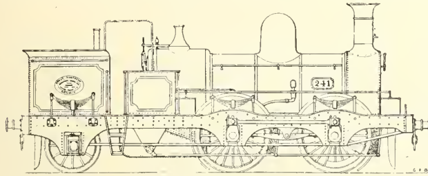
FIG. 197—A STURROCK'S TANK ENGINE FOR THE G.N.R., BUILT BY THE AVONSIDE ENGINE CO., 1865
