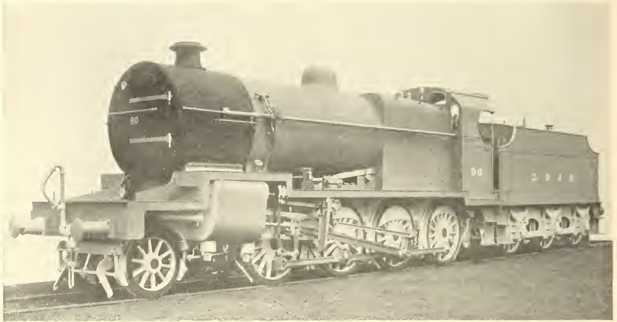
FIG. 446—SIR H. FOWLER'S EIGHT-COUPLED GOODS ENGINE, SOMERSET & DORSET JOINT RLY., 1925
