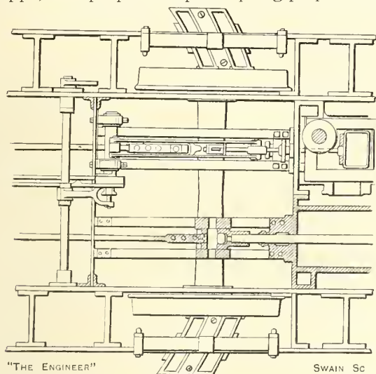
FIG. 207—W. BRIDGES ADAMS'S RADIAL AXLE, 1863
