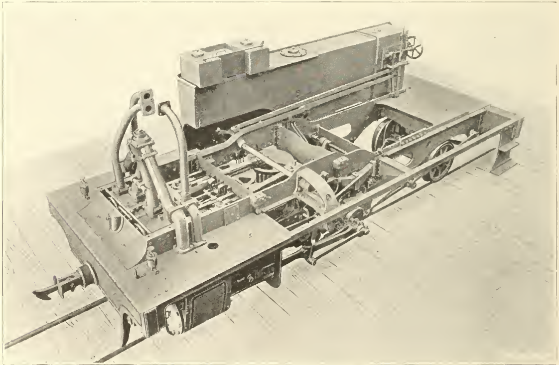
FIG. 402—FRAME, MOTION AND GEARING OF FELL'S CENTRAL RAIL SYSTEM ENGINE. BY NEILSON & CO., FOR NEW ZEALAND, 1886
