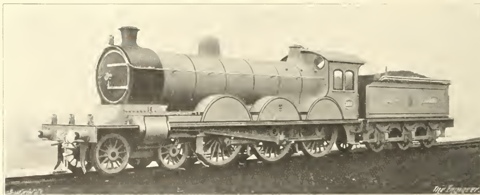
FIG. 385—W. WORSDELL'S 4-6-0 EXPRESS ENGINE. "2111" CLASS, NORTH-EASTERN RLY., 1900-1
