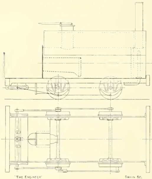
FIG. 156—NEILSON'S SINGLE CYLINDER ENGINE, 1857
