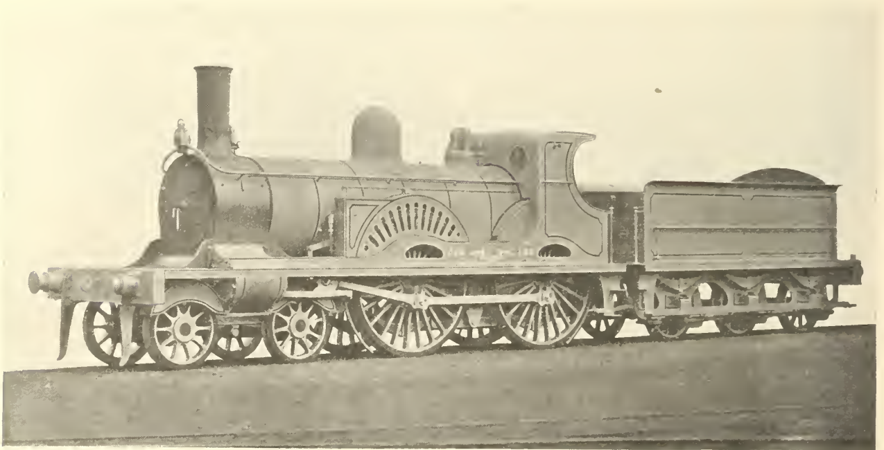
FIG. 280—BRITTAİN'S 4-4-0 PASSENGER ENGINE, CALEDONIAN RAILWAY, 1877
