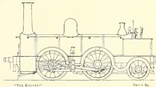
FIG. 146—P. STIRLING'S G. & S.W. RLY. ENGINE, 1857
