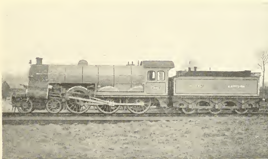
FIG. 440—STUMPF UNIFLOW CYLINDER LOCOMOTIVE, NORTHEASTERN RLY., 1913
