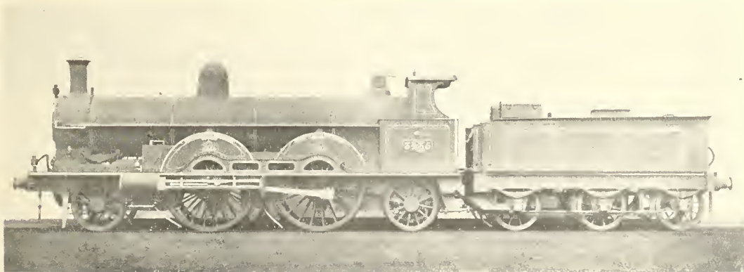
FIG. 365—F. W. WEBB'S THREE-CYLINDER COMPOUND ENGINE, "GREATER BRITAIN" CLASS, L. & N.W. RLY., 1891
