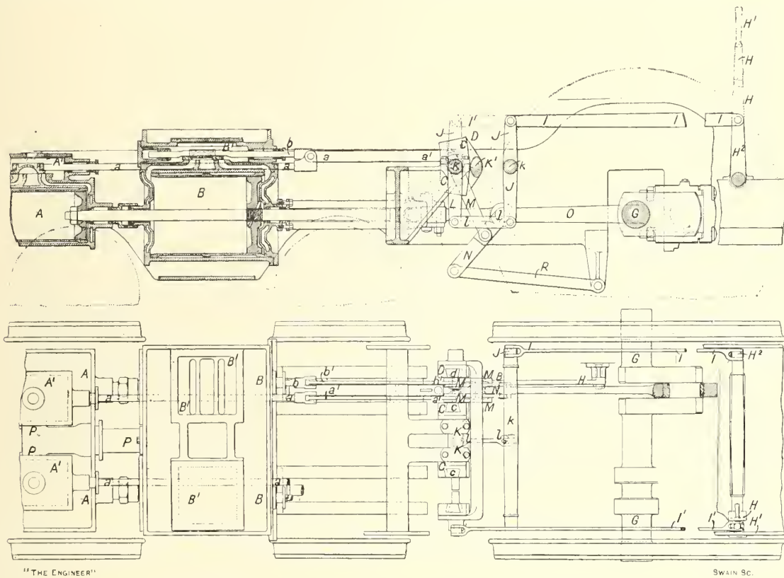
FIG. 322.—NESBIT'S FOUR-CYLINDER TANDEM COMPOUND ENGINE, N.E.R., 1885
