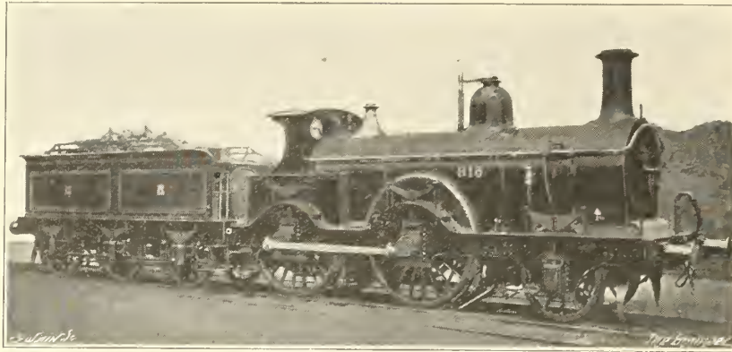
FIG. 245—M. KIRTLEY'S 800 CLASS EXPRESS LOCOMOTIVE, MIDLAND RLY., AS REBUILT 1875-82
