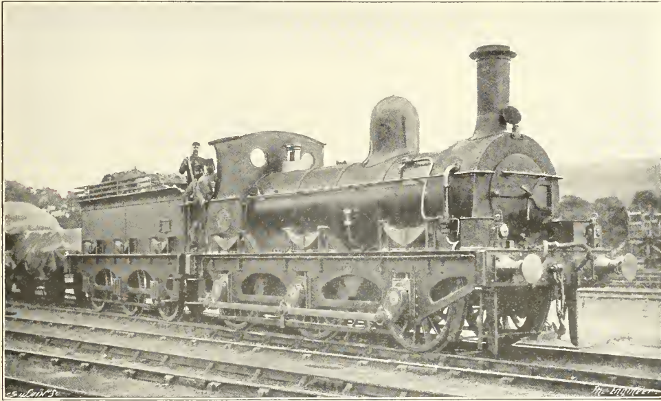
FIG. 290—C. SACRE'S M.S. AND L.R. HEAVY GOODS ENGINE, 1880-85 (Photo. Locomotive)
