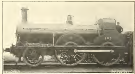
FIG. 274—H. SMELLIE'S G. & S.W.R. ENGINE, 1879-80
