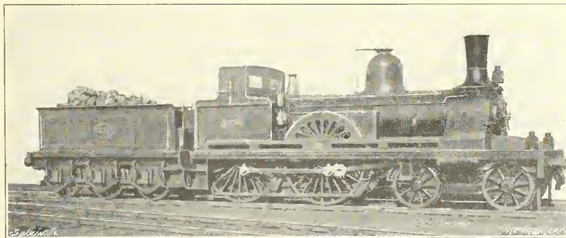
[Photo. Locomotive
